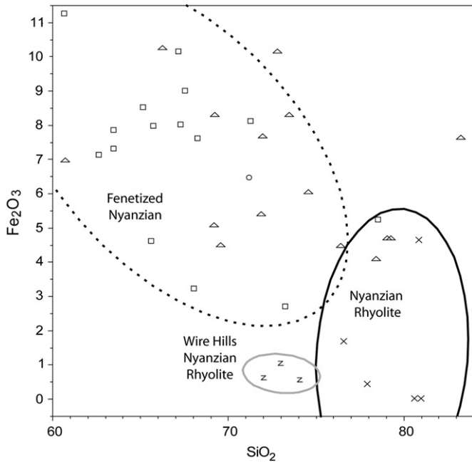
Fig. 7. Comparison of SiO 2 % and (Fe 2 O 3 %) for fenetized Nyanzian samples and other primary source samples. Ellipses represent 3 sigma intervals. Wire Hills rhyolite primary source samples are depicted as “z”s. Fenetized Nyanzian secondary samples are depicted as triangles. Nyanza rhyolite primary source samples are depicted as “x”s. Fenetized Nyanzian primary source samples are depicted as boxes. Fenetized Nyanzian artifact sample is depicted as an open circle.
