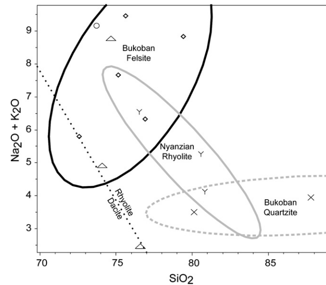
Fig. 15. Comparison of total alkali (K 2 O % + Na 2 O %) and silica SiO 2 % for Bukoban felsite primary source samples and other primary source samples. Ellipses represent 3 sigma intervals. Bukoban quartzite primary source samples are depicted as “x”s. Nyanzian rhyolite primary source samples are depicted as “y”s. Bukoban felsite primary source samples are depicted as diamonds. Bukoban felsite secondary samples are depicted as open triangles. The Bukoban felsite artifact sample is depicted as an open circle.
