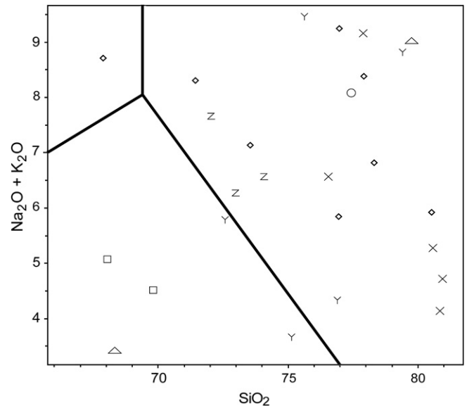
Fig. 13. Comparison of total alkali (K 2 O + Na 2 ) and silicon (SiO) in Ouygis granite primary source samples and other primary source samples. Nyanzian rhyolite primary source samples are depicted as "x"s. Wire Hills rhyolite primary samples are depicted as "z"s. Bukoban felsite primary source samples are depicted as "y"s. Ouygis granite primary samples are depicted as diamonds. Miriu granodiorite primary samples are depicted as boxes. Ouygis granite secondary samples are depicted as open triangles. Ouygis granite artifact sample is depicted as an open circle.
