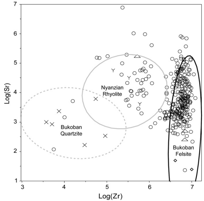
Fig. 16. Comparison of the logarithmic transformation of strontium (ppm) and zirconium (ppm) values for Bukoban felsite primary source samples and other primary source samples. Ellipses represent 3 sigma intervals. Bukoban quartzite primary source samples are depicted as “x”s. Nyanzian rhyolite primary source samples are depicted as “y”s. Bukoban felsite primary source samples are depicted as diamonds. Bukoban felsite secondary samples are depicted as open triangles. The Bukoban felsite artifact sample is depicted as open circles.
