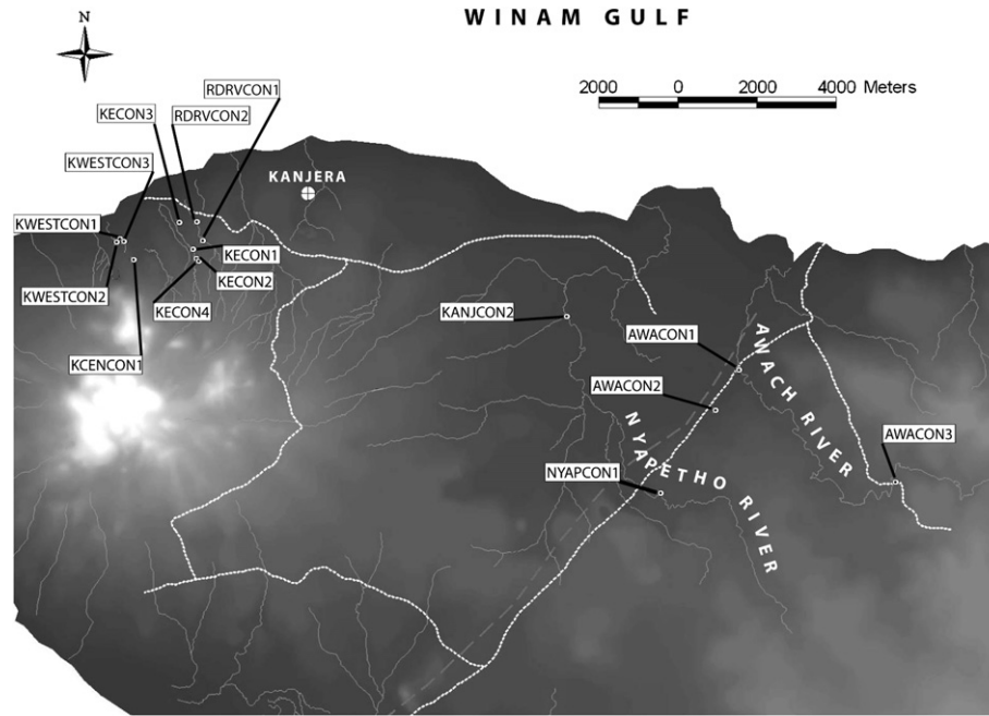
Fig. 20. Map of conglomerates sampled in this study.
